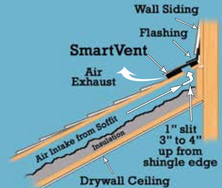
Roof to Wall Exhaust
